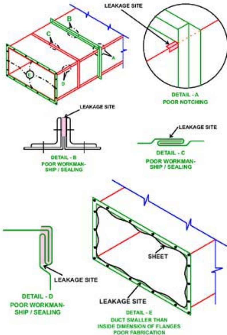
Figure 1 : Common duct leakage sites
