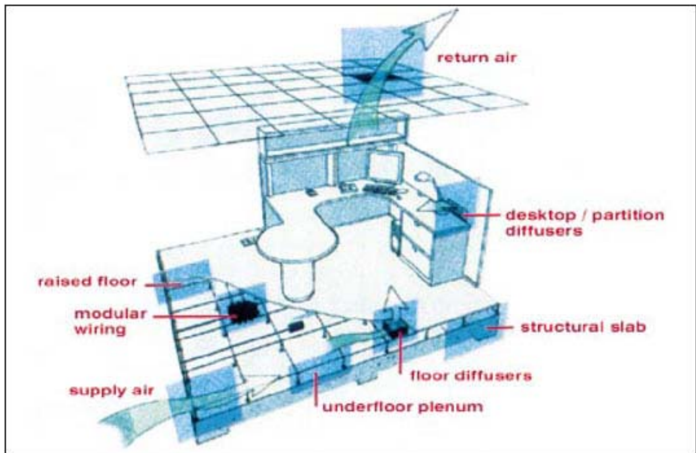
Figure 1 : Cutaway of typical office work space with underfloor air distribution.
