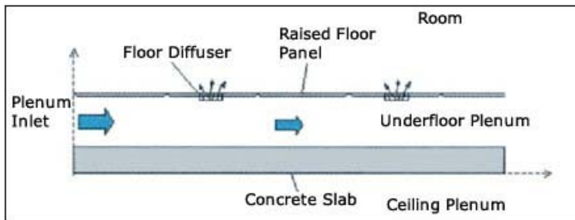
Figure 3 : Underfloor plenum schematic
