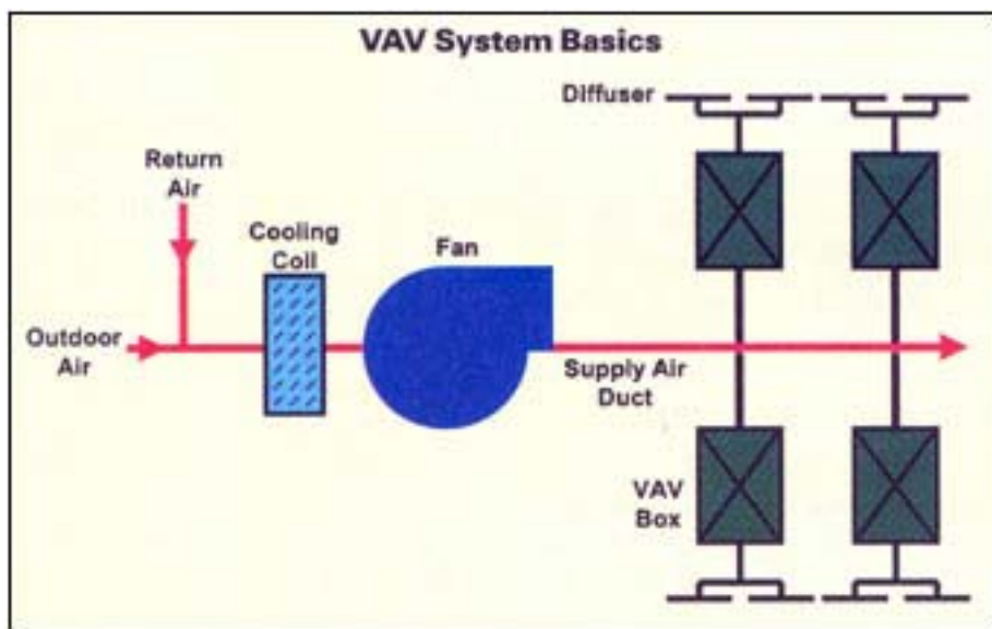
Fig 1 – Simplified Schematic of a VAV System
