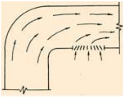
Figure 6 : Outlet too close to elbow
